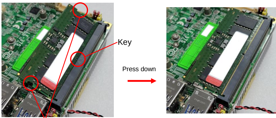
Mounting notch
