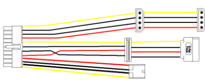
Power Cable x 1 (OALATX-P3S2)
