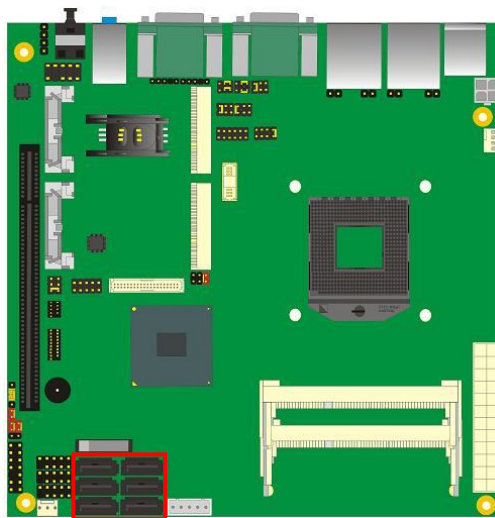
SATA6 SATA3 SATA5 SATA2 SATA4 SATA1
