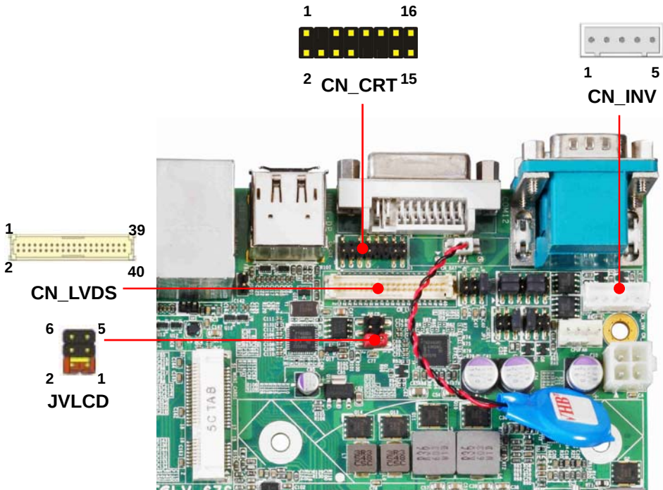
CN_CRT: VGA 16-pin connector (Pitch 2.00 mm)
