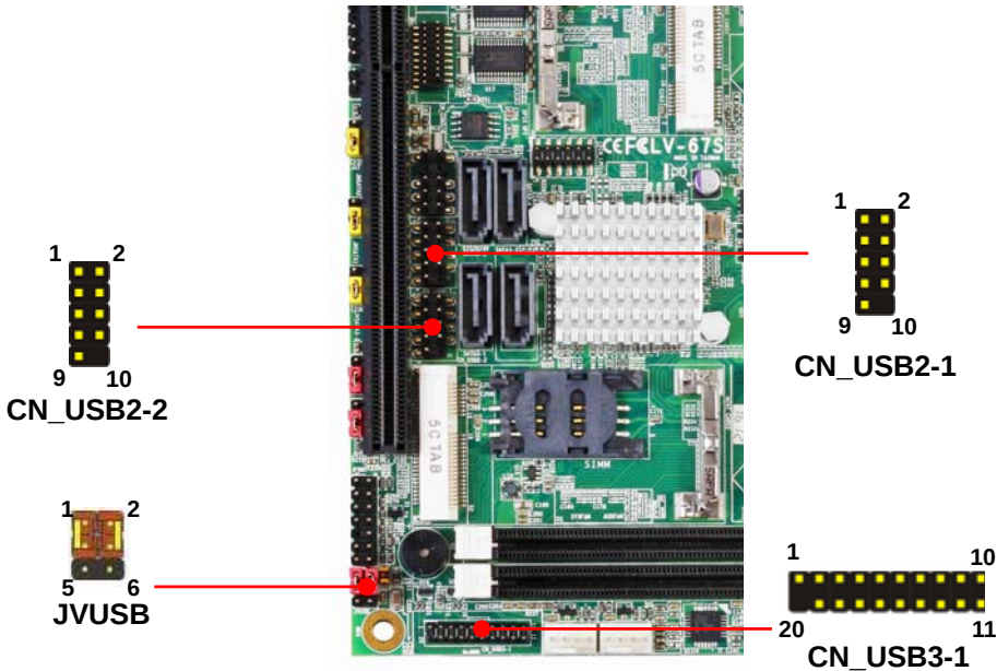
CN_USB 2-1/2-2: USB2.0 10-pin header (Pitch 2.54 mm)
