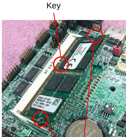
Mounting notch
