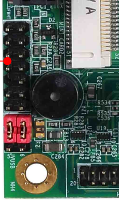
JFRNT: Front panel switch and indicator 14-pin header (Pitch 2.54mm)
